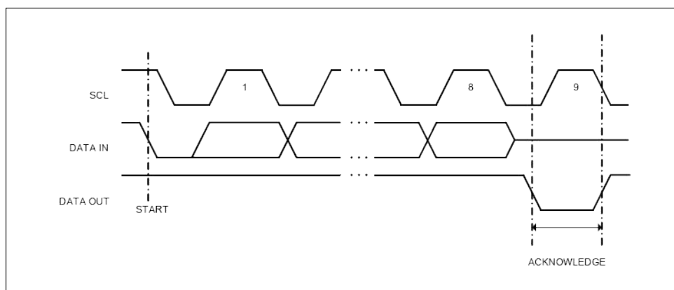
Figure 3:Output Acknowledge
