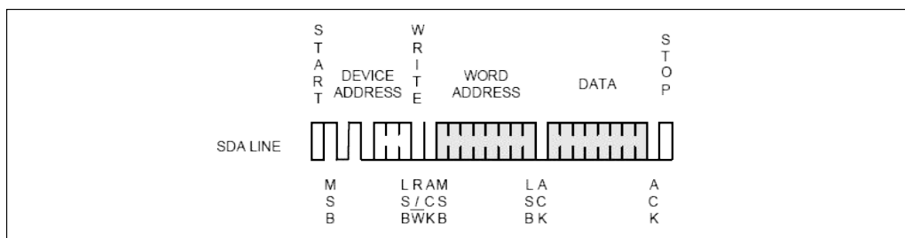
Figure 6: Page Write
