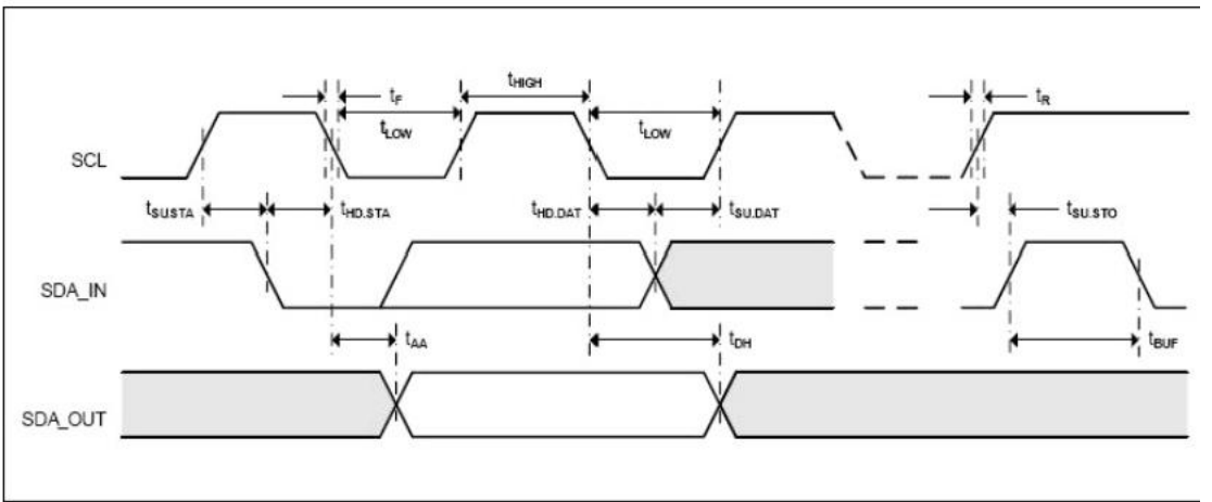
Figure 10: SCL: Serial Clock, SDA: Serial Data VO
