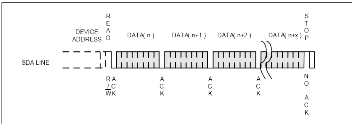
Figure 9:Sequential Read
