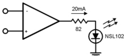
LED Driver
