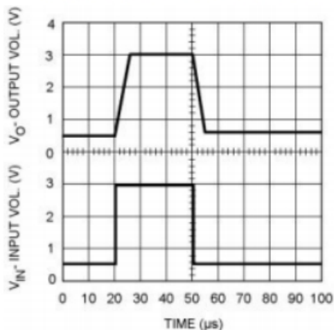
Sinking Current
