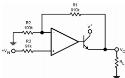
Power Amplifier
