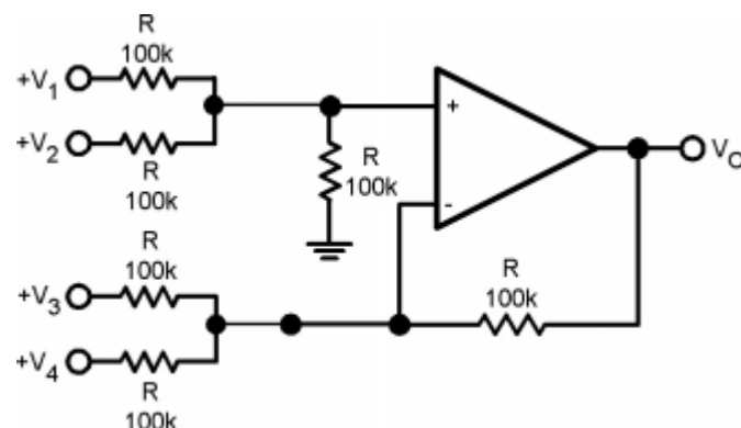
DC Summing Amplifier (V)
