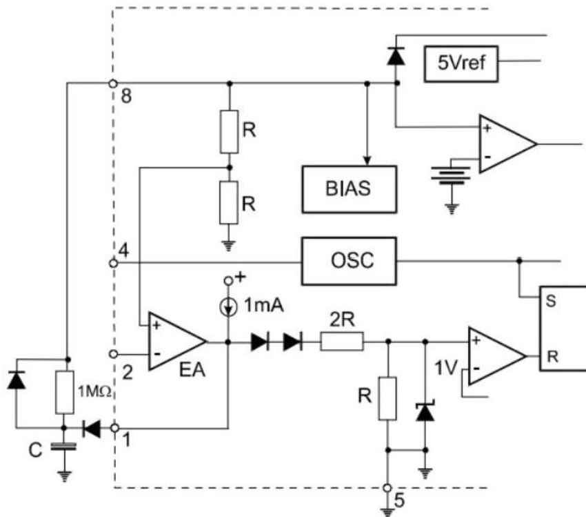
Figure 8. Soft-Start Circuit
