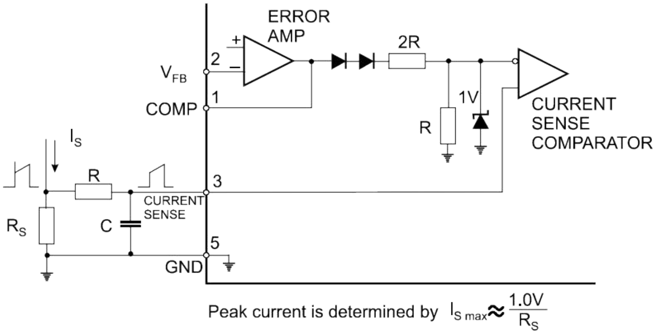
Figure 3. Current Sense Circuit
