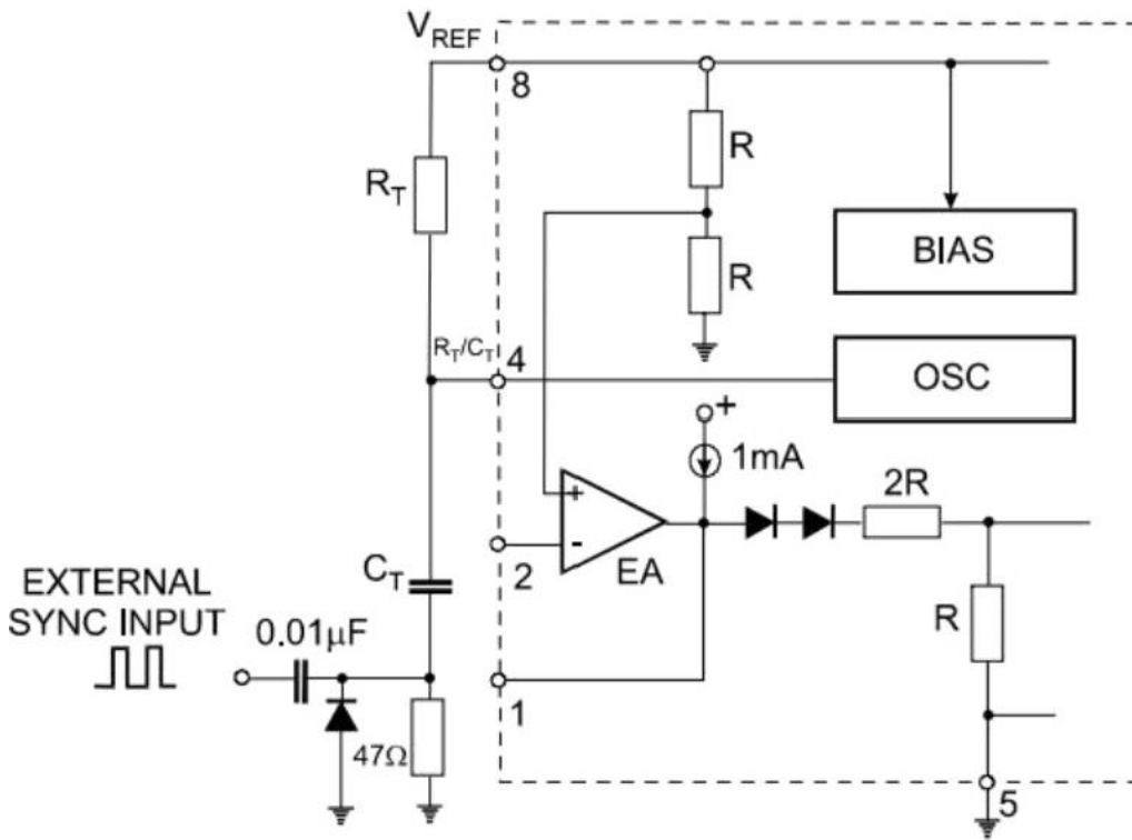
Figure 7. External Clock Synchronization
