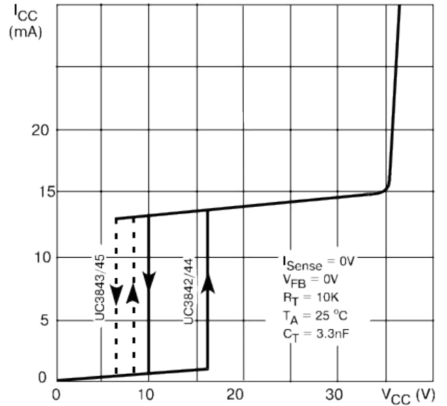
Figure 8. Supply Current vs. Supply Voltage
