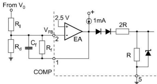
Figure 5.Latched Shutdown
