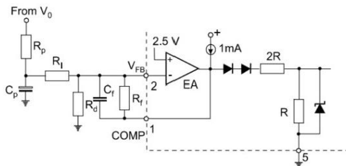
Figure 6.Error Amplifier Compensation
