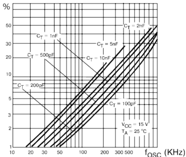
Figure 2. Output Dead-Time vs. Oscillator Frequency
